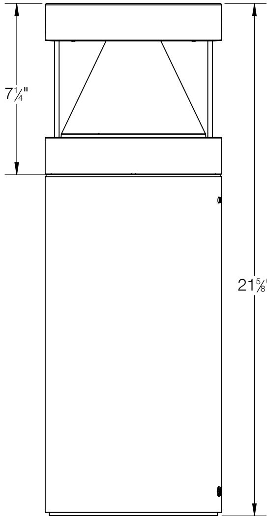
99856 SYSTEM BOLLARD HEAD SHOWN ON SYSTEM BOLLARD TUBE 99615 (NOT TO SCALE, TUBE SOLD SEPERATELY)
