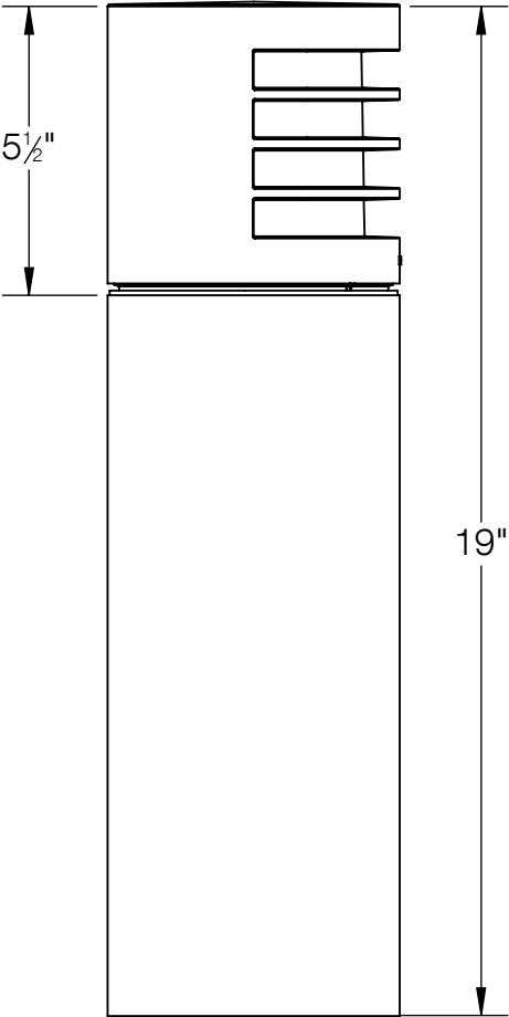
99770 SYSTEM BOLLARD HEAD SHOWN ON SYSTEM BOLLARD TUBE 99614 (NOT TO SCALE, TUBE SOLD SEPERATELY)
