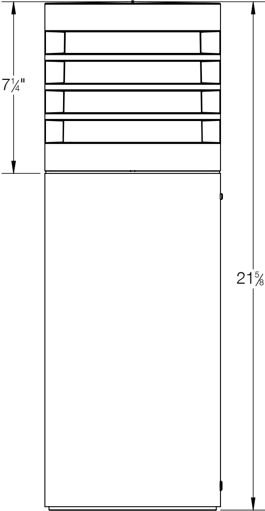
99765 SYSTEM BOLLARD HEAD SHOWN ON SYSTEM BOLLARD TUBE 99615 (NOT TO SCALE, TUBE SOLD SEPERATELY)
