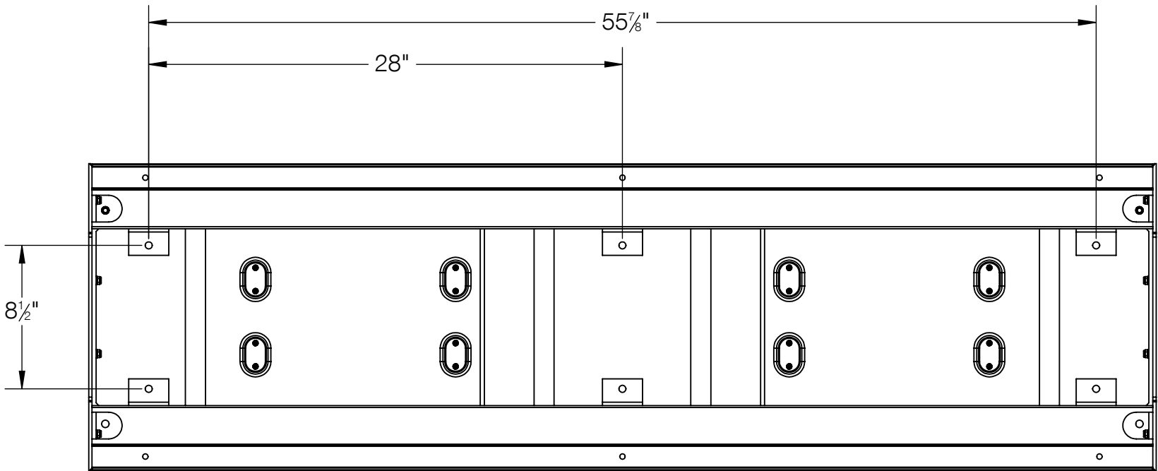
BACK VIEW (MOUNTING DETAIL)
