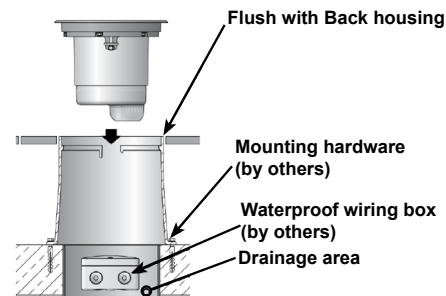
Figure 2: Faceplate Detail
