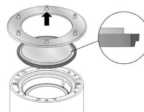
Figure 4: Faceplate Removal (Generic Image)
