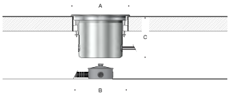
In-grade luminaire · Adjustable · Very wide beam
