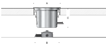
In-grade luminaire · Adjustable · Focused beam
