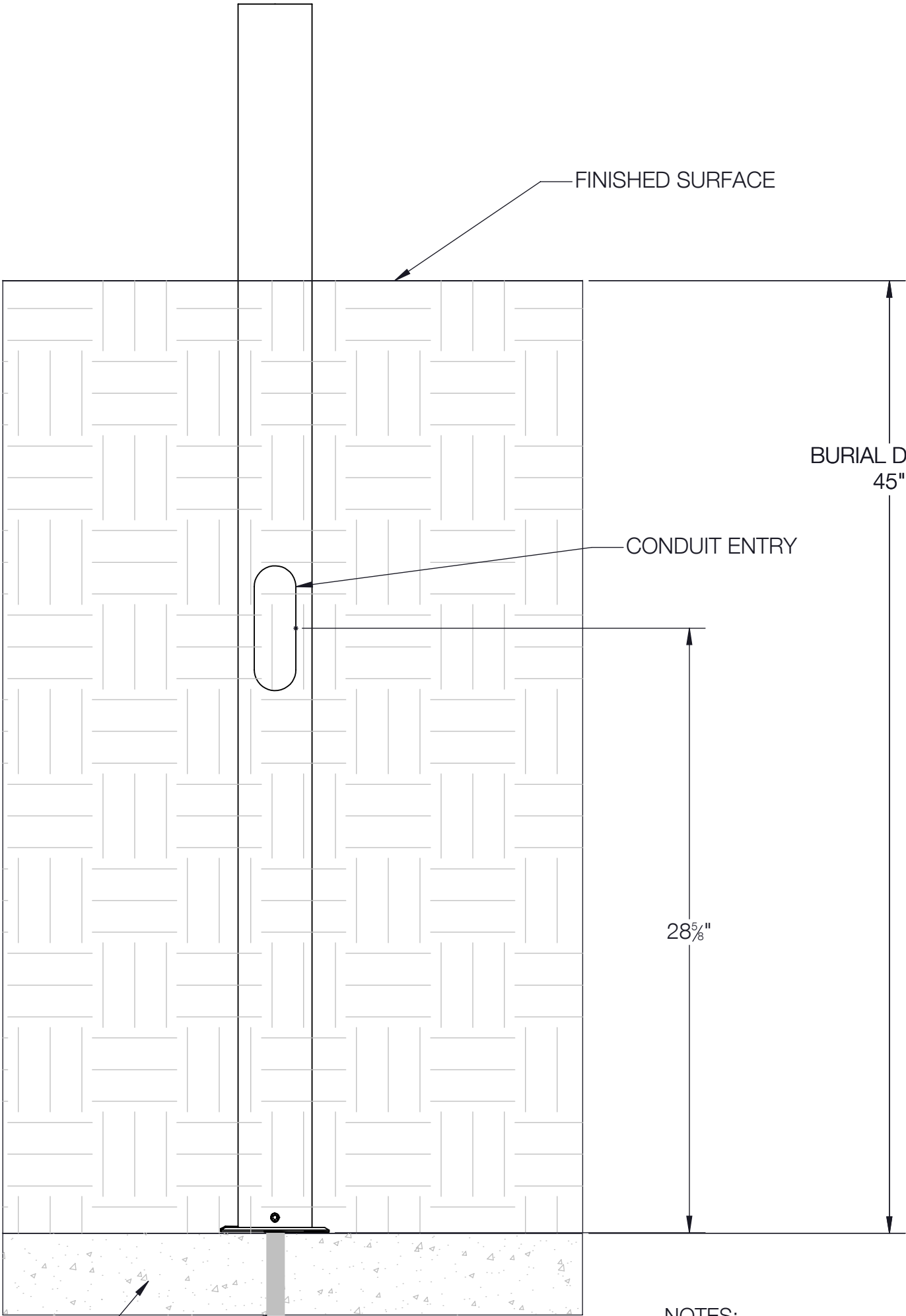
SUB-BASE
