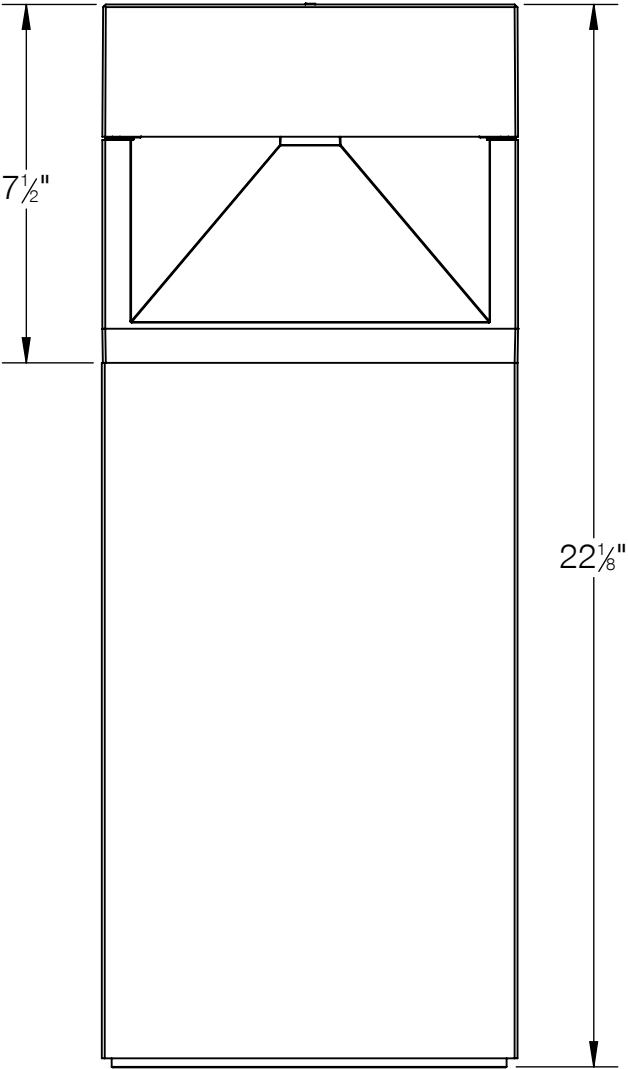
84691 SYSTEM BOLLARD HEAD SHOWN ON SYSTEM BOLLARD TUBE 84001 (NOT TO SCALE, TUBE SOLD SEPERATELY)
