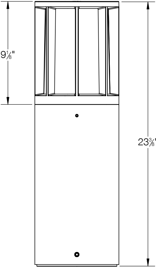
84683 SYSTEM BOLLARD HEAD SHOWN ON SYSTEM BOLLARD TUBE 99615 (NOT TO SCALE, TUBE SOLD SEPERATELY)
