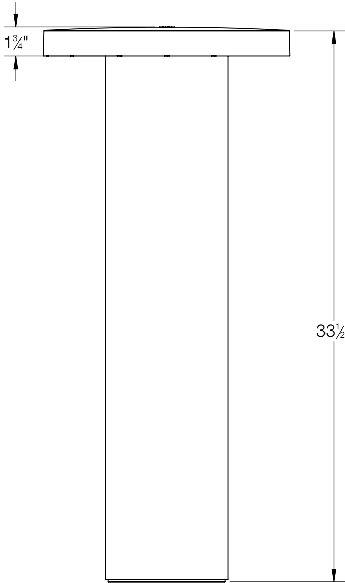
84642 SYSTEM BOLLARD HEAD SHOWN ON SYSTEM BOLLARD TUBE 99653 (NOT TO SCALE, TUBE SOLD SEPERATELY)
