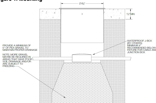
Figure 1: Mounting
