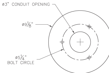
Figure 1: Anchorage Template
