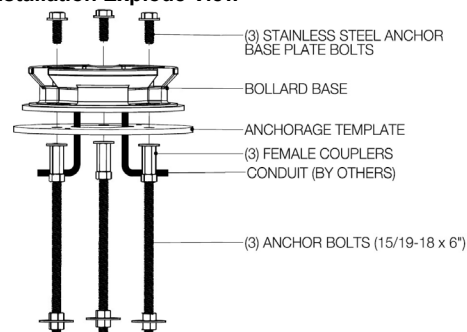
Figure 2: Installation Explode View
