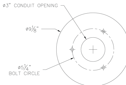
Figure 1: Anchorage Template
