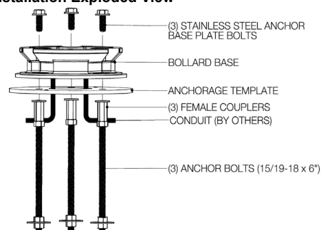
Figure 2: Installation Exploded View
