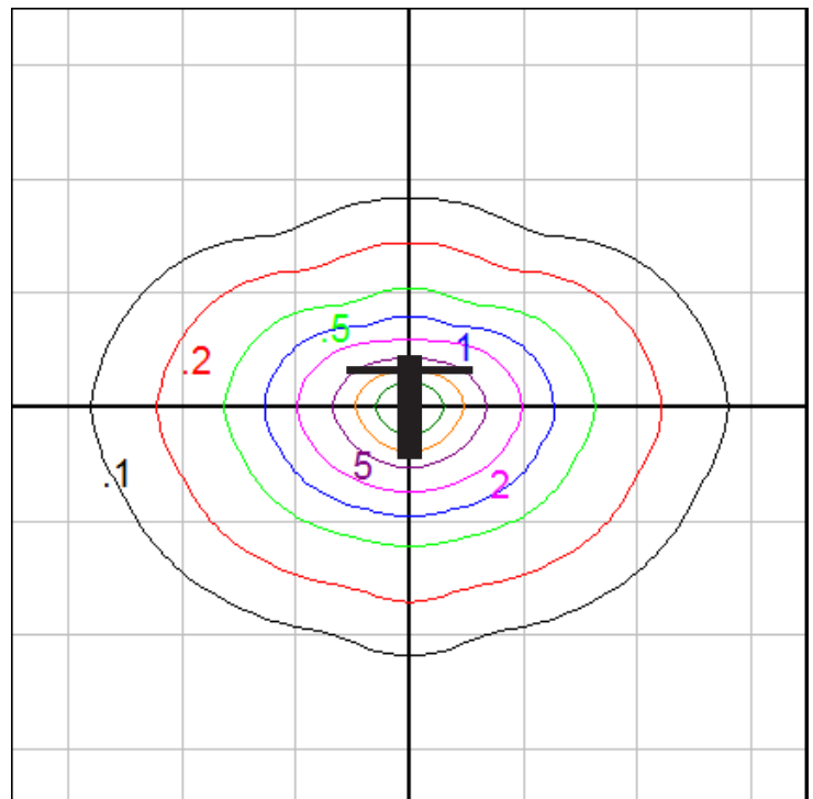
Wall Mount - Isogrid on Wall Grid Spacing = 2.5 ft.
