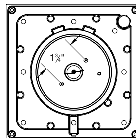
Figure 2: Luminaire back with round wall mount casting
